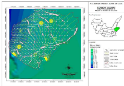
Figure 4. Groundwater contour map for Tarawang District in Jeneponto Regency
